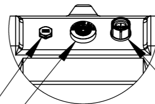
PRV Option Gore Membrane Vent — PRV Option AGM Breather Valve — PRV Option Humidity Indicator
