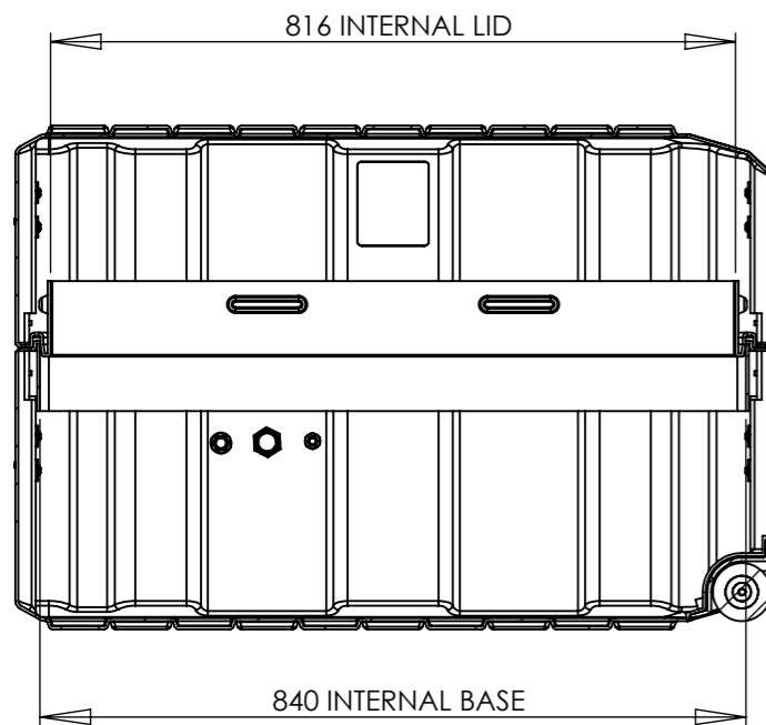
SECTION Y-Y
