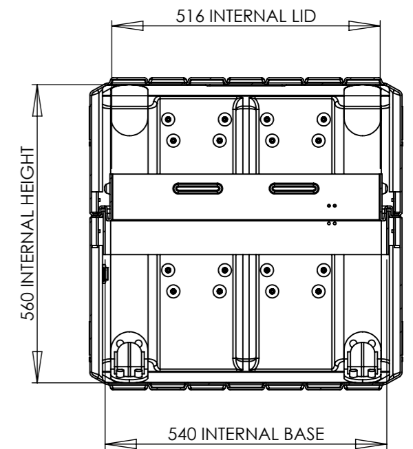
SECTION Z-Z
