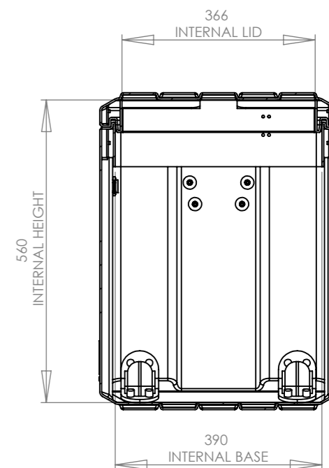
SECTION Z-Z
