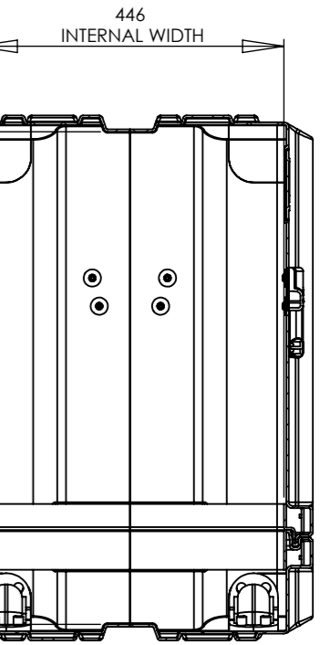
SECTION Z-Z SCALE 1 : 10
