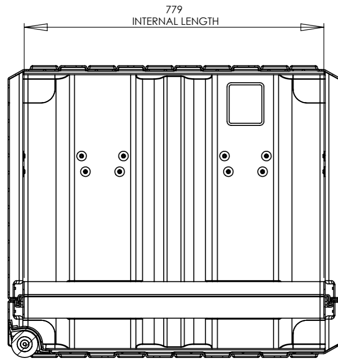
SECTION Y-Y SCALE 1 : 10
