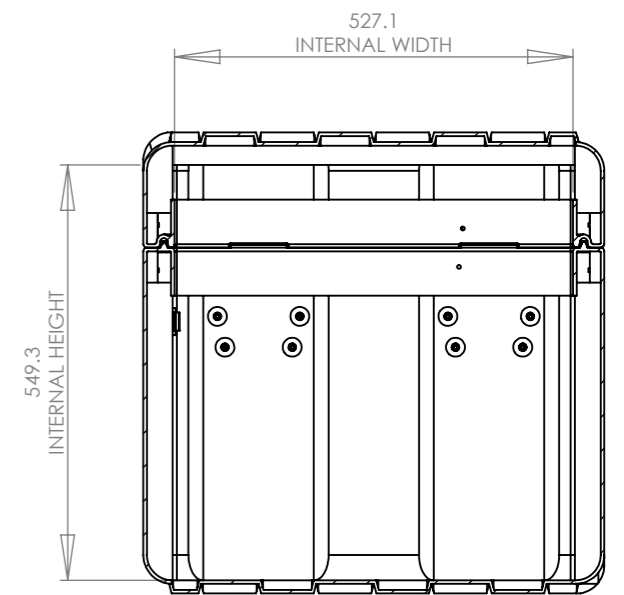
SECTION Z-Z
