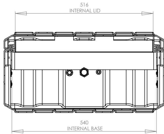
SECTION Y-Y SCALE 1 : 7
