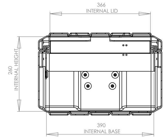
SECTION Z-Z SCALE 1 : 7
