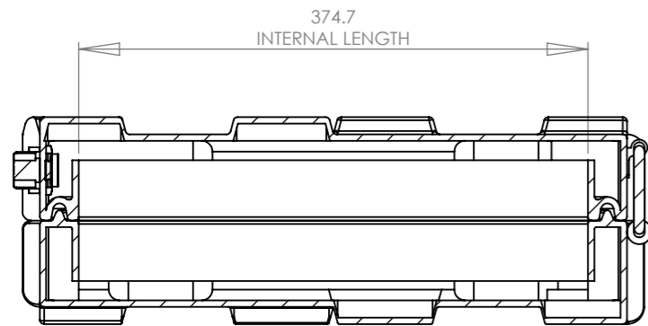
SECTION Y-Y
