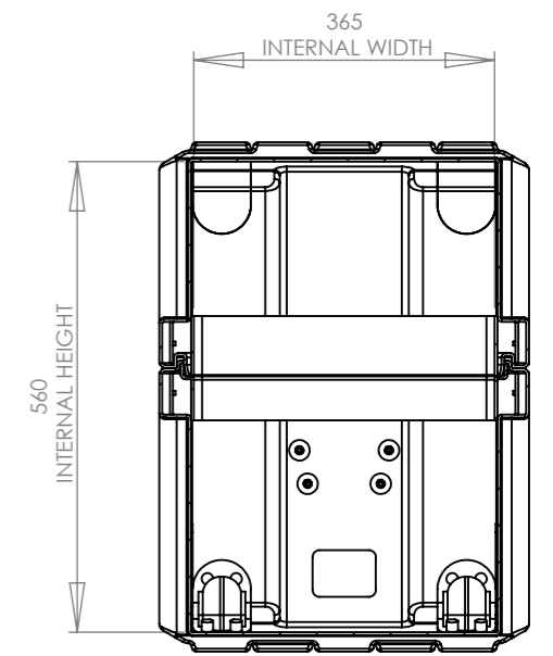
SECTION Z-Z
